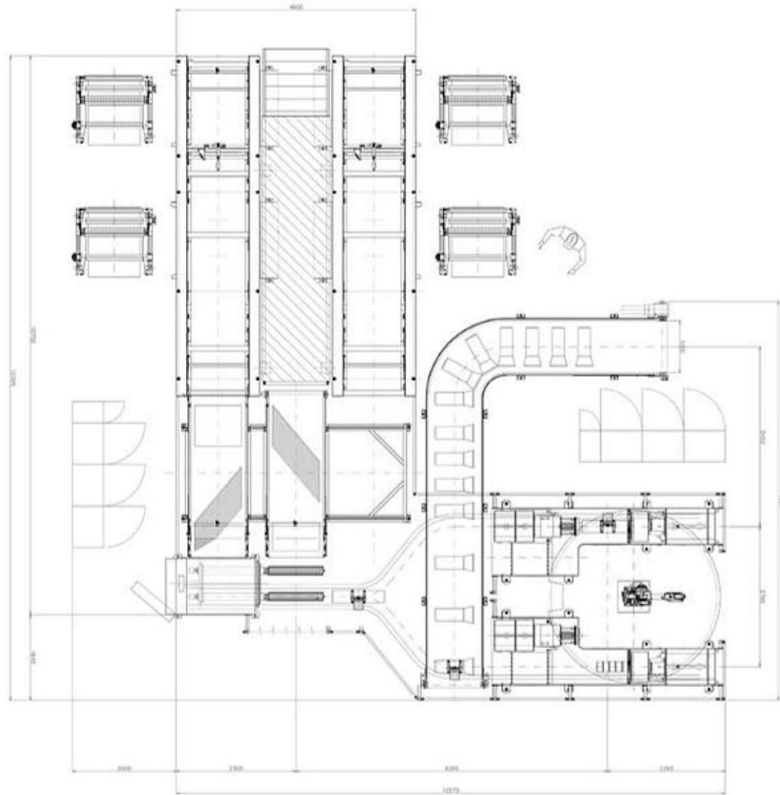
Above: Intereuropean's fully automatic air-spring building system
