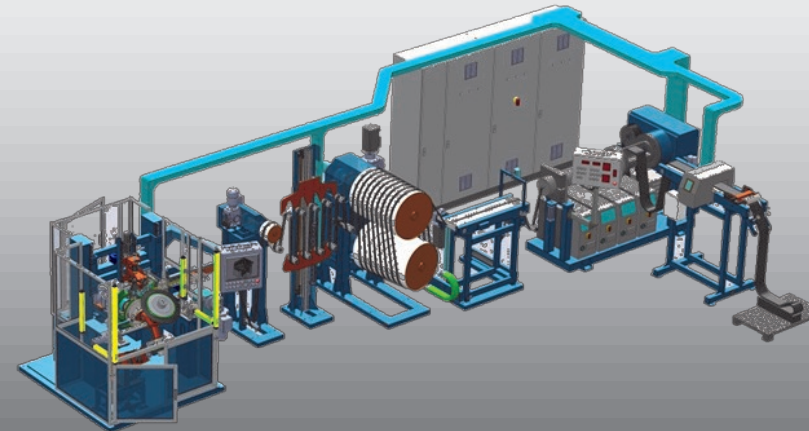
Bead Apexing Line 13" - 20" with cold feed apex extruder
