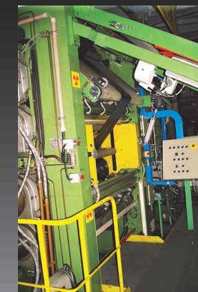
Rubber Calender Line with IL+PLY preassembling
