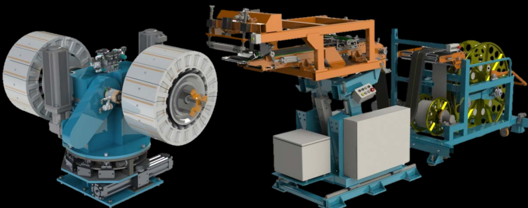
2nd Stage TBM Upgrade Twin Drums Turret
