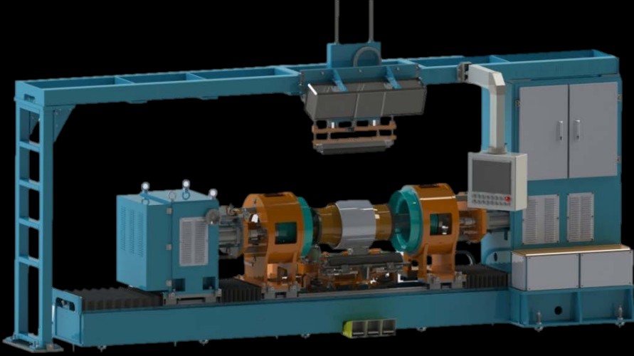
1st Stage TBM Upgrade Bladder turn-up system
