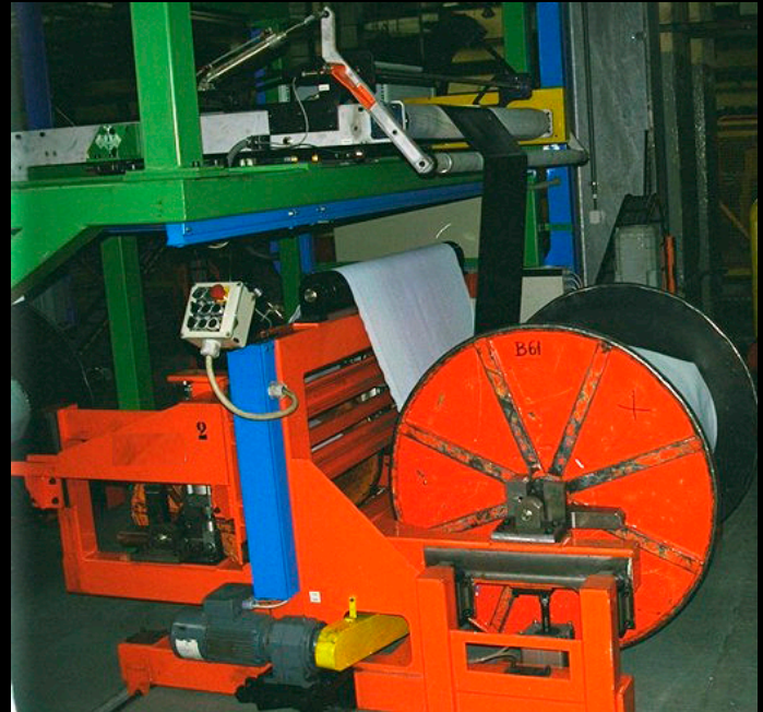
New Wind-up stations for Calender/Extrusion Lines
